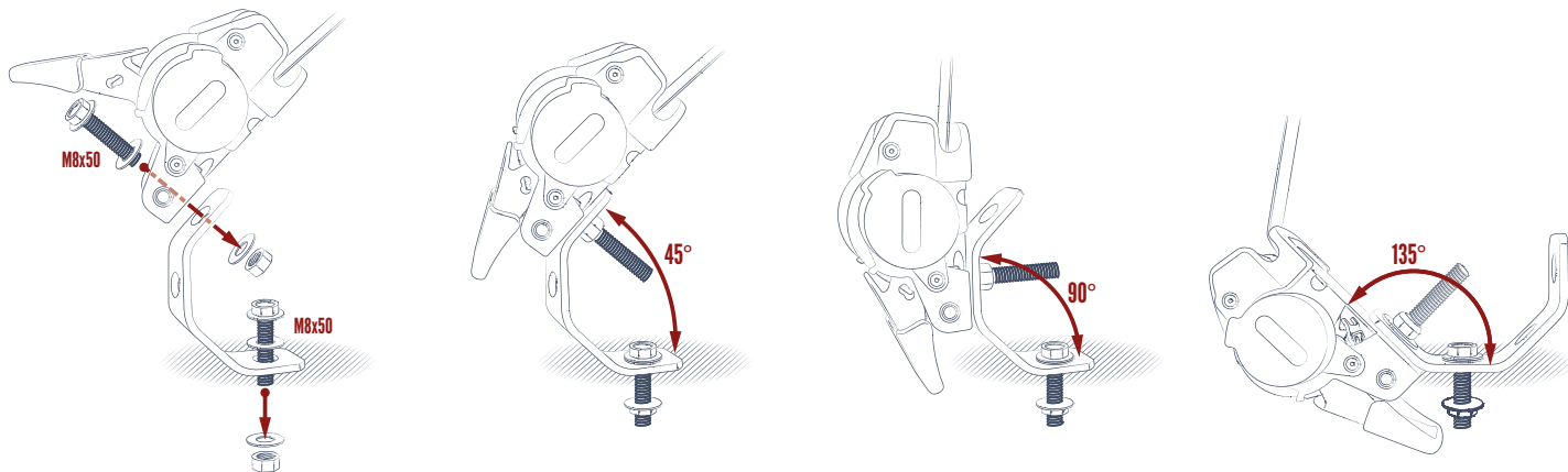
Different possible installation angles for the tensioner
